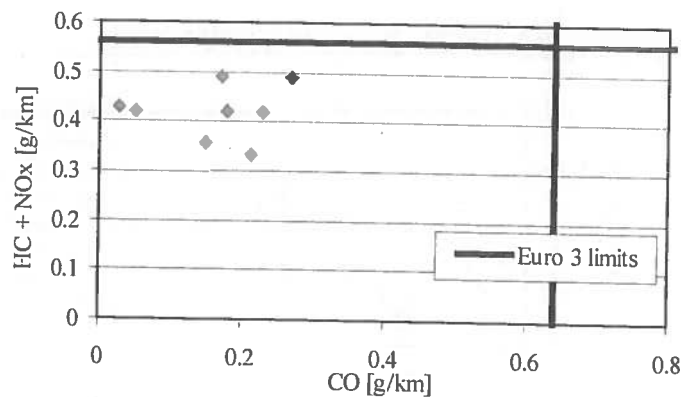
Figure 10: Diesel CO and HC+NO x , EURO 3
