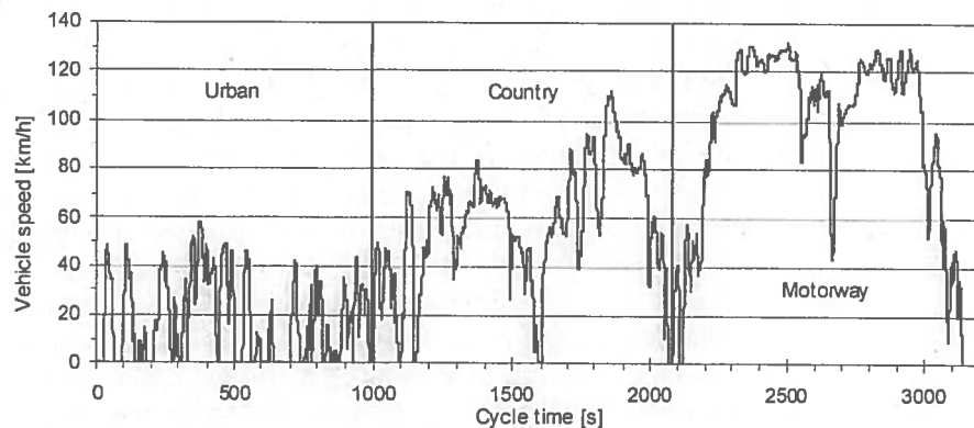
Figure 2: CADC (Common Artemis Driving Cycle)
