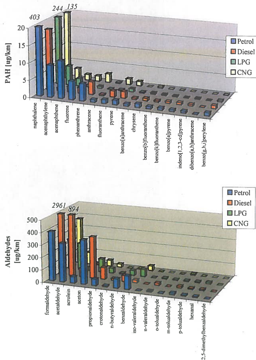
Emissions and emission profiles: Average driver
