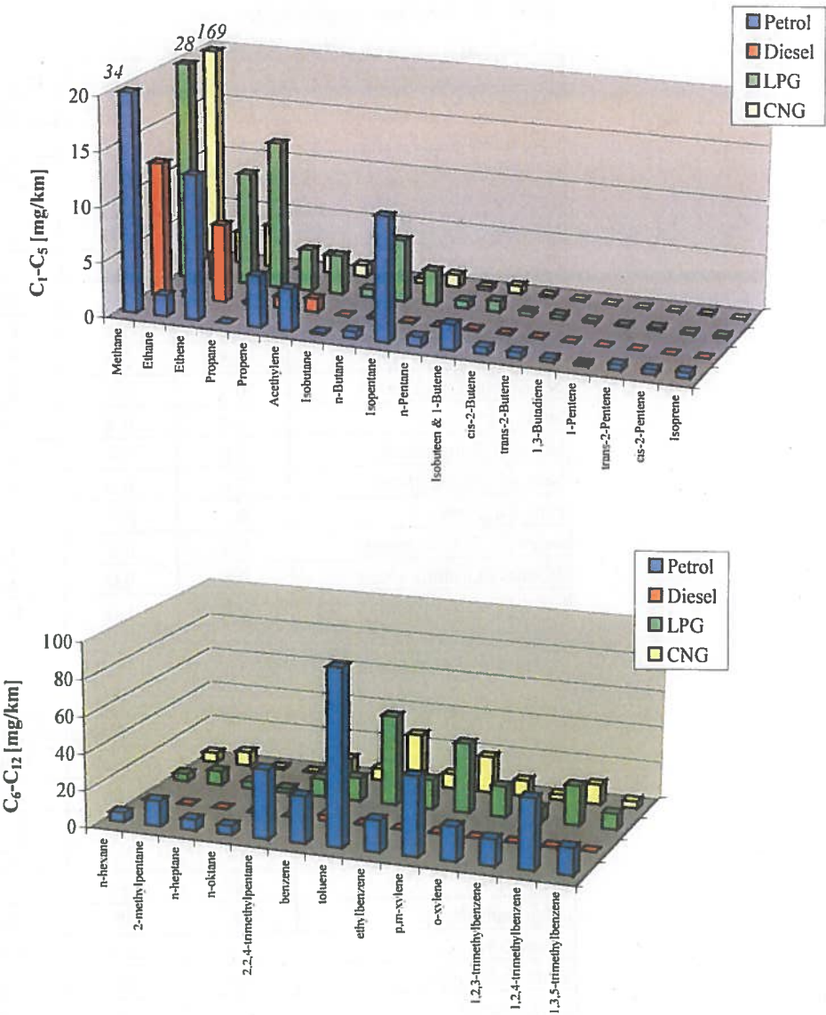
Figure 42: C 1 -C 12 emission profile
