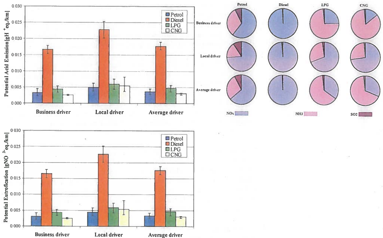
Figure 20: The measured or calculated ecological effect indicators (bars) and the relative weighed contributions of the components involved to the calculation (pies)
